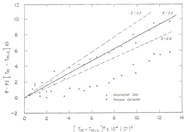
FIG. 3. Normalized melting pressure as a function of the square of the increase in melting temperature. This curve is used in the determination of the Simon equation parameter.
