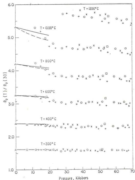
FIG. 5. Resistance of gold at temperature T to that at 30^\circ\text{C} as a function of pressure. The solid line follows the calculated initial slope at zero pressure and the dashed line is the calculated curve after a vacancy correction is made.
